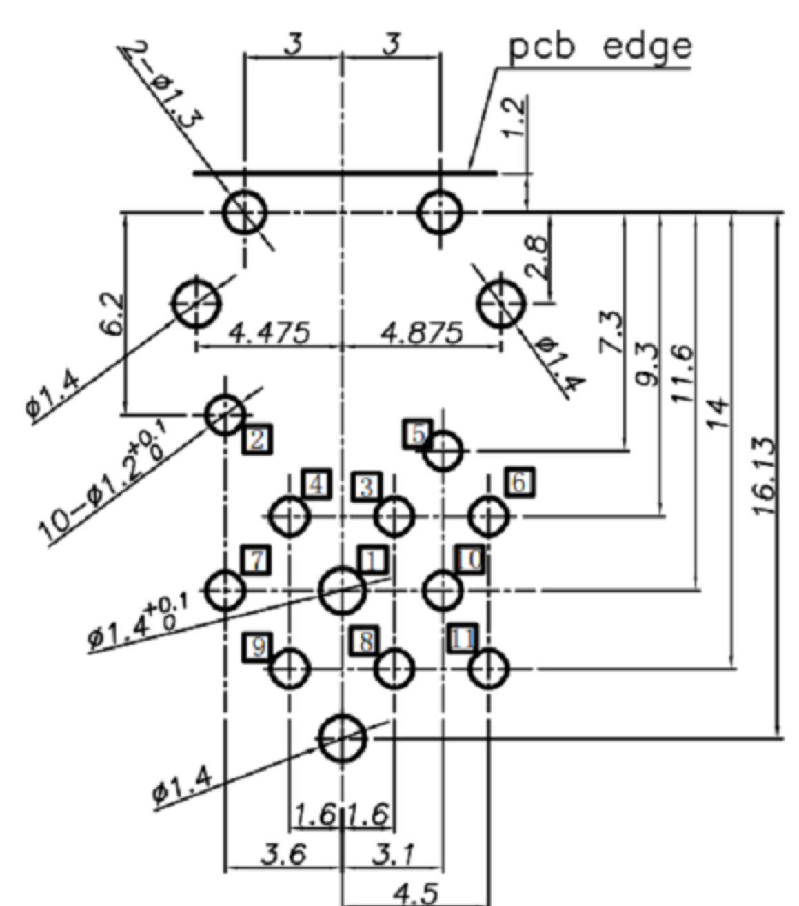
RECOMMENDED P. C. B. LAYOUT UNSPECIFIED TOLERANCE: ±0.05 (TOP VIEW)
