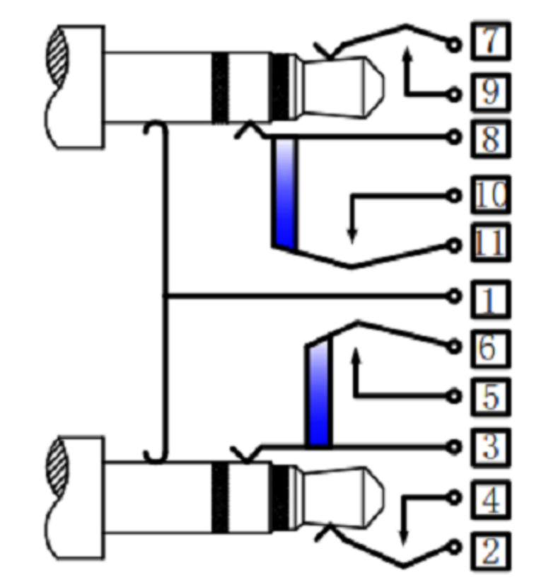
PLUG inserted
